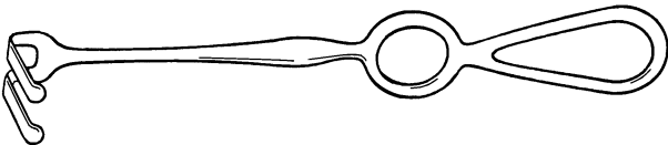
16295-13 Ollier Retractor, single ended, 2 prong, 240mm, 13mm wide x 20mm deep blade
