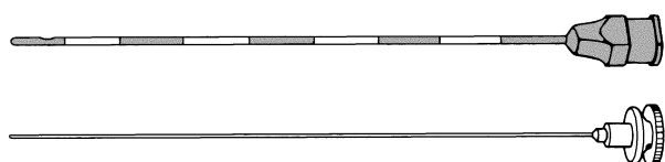
71300-14 Cone Ventricular Cannula, graduated in cms, luer fitting, 2.03mm diameter (14 swg) 71300-16 Cone Ventricular Cannula, graduated in cms, luer fitting, 1.63mm diameter (16 swg) 71300-18 Cone Ventricular Cannula, graduated in cms, luer fitting, 1.22mm diameter (18 swg)
