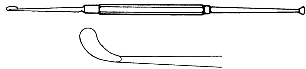
35130-19 Freer Nasal Knife, curved to side, 190mm
